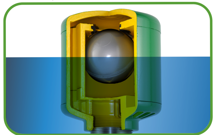
closed position
