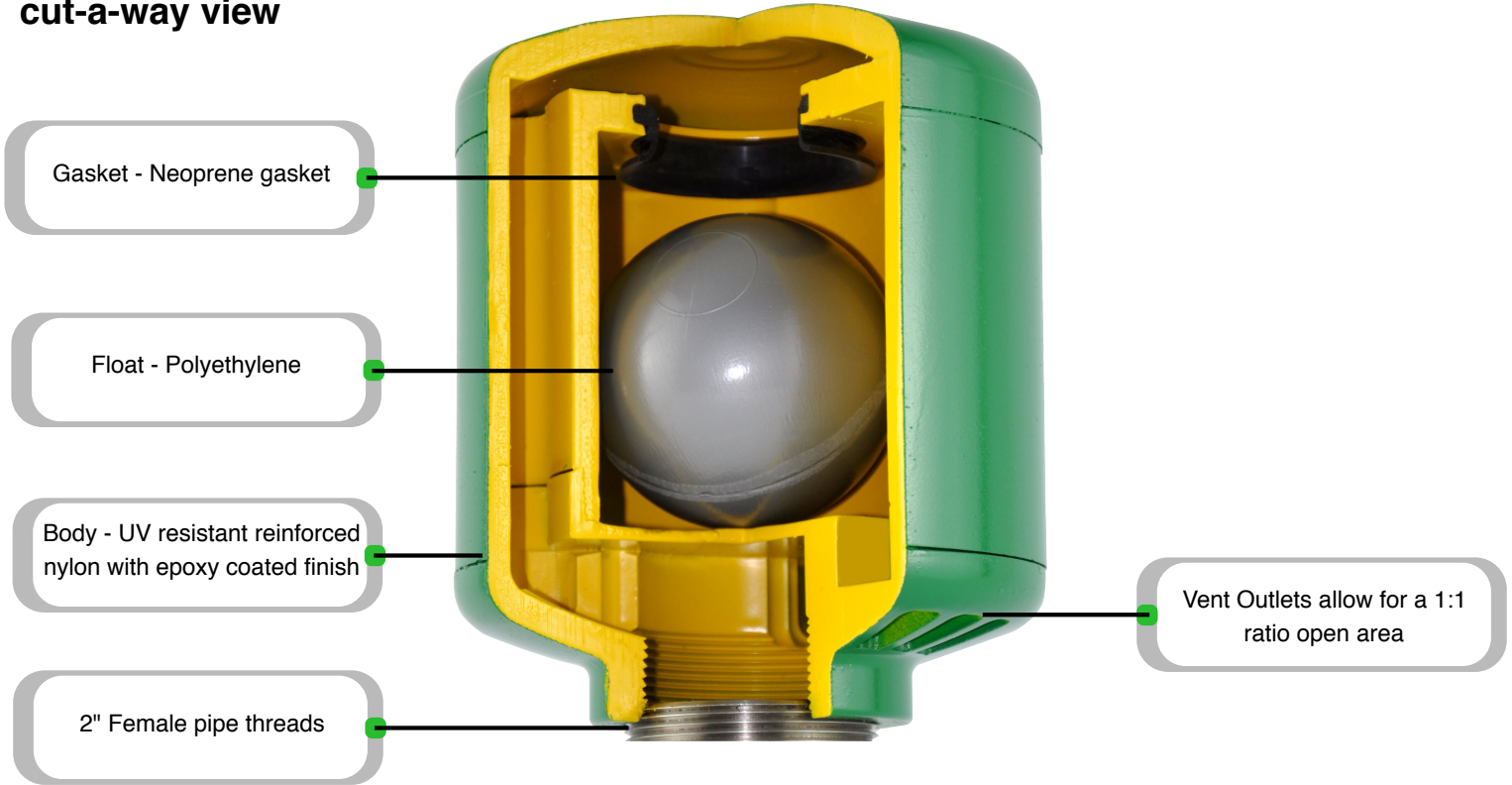
open position
