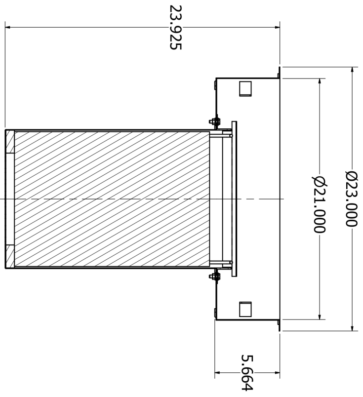
SECTION A-A SCALE 1 / 4
