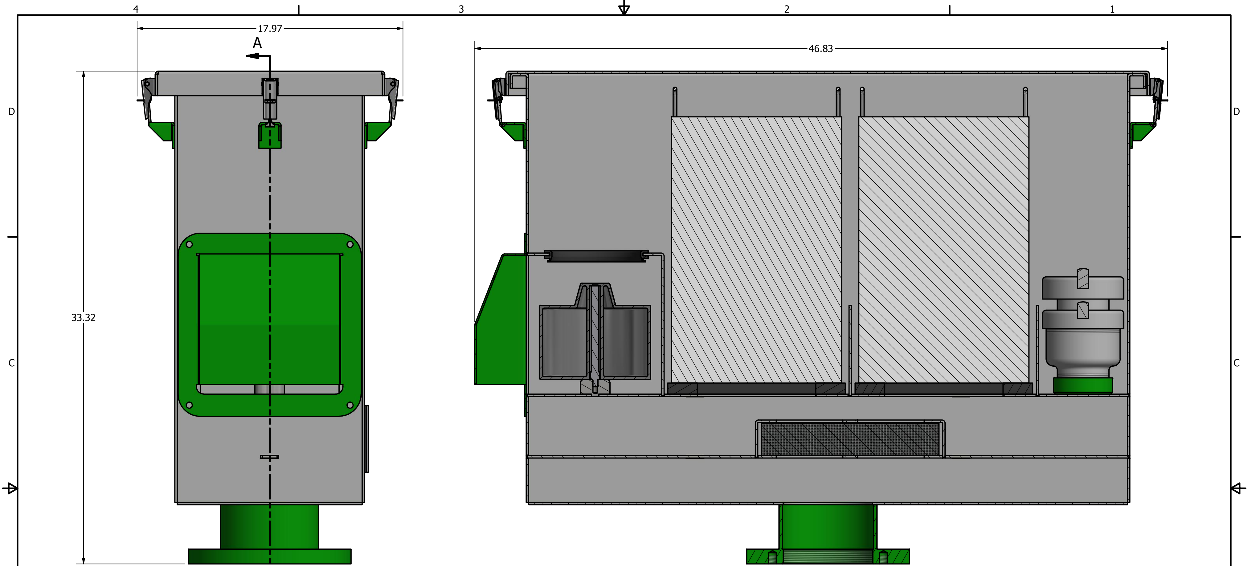
SECTION A-A SCALE 1 / 4
